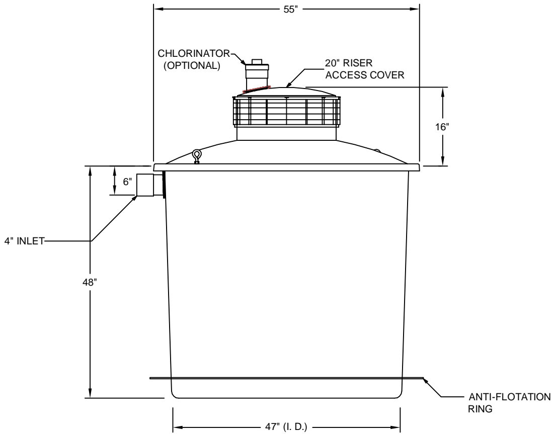
SIDE VIEW
