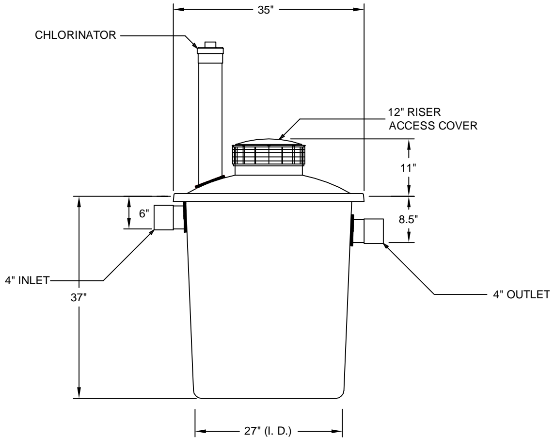
SIDE VIEW
