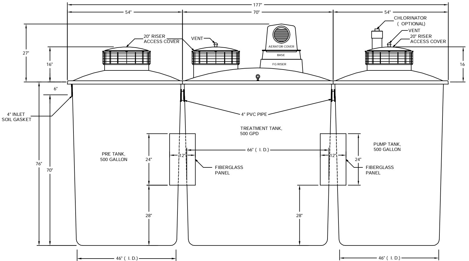
SIDE VIEW
