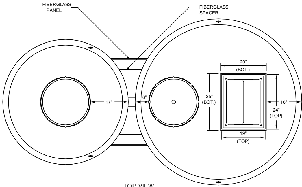
TOP VIEW
