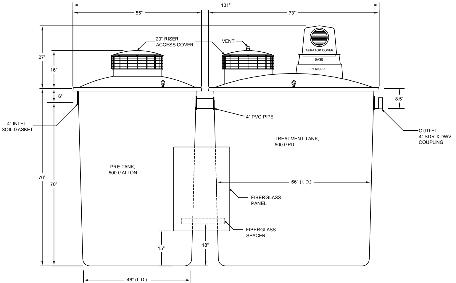
SIDE VIEW
